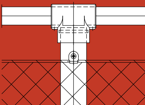
Bajonetsluiting in detail
